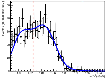
Passed DiF (before RICH1) ( 0 < n_{\text{Tracks}} < 200 , 3.6 < \eta < 5.0 , 15600 < p < 27000 )
