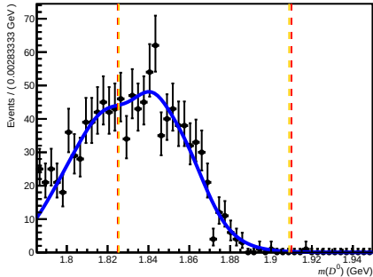
Passed DiF (before RICH1) ( 0 < n_{\text{Tracks}} < 200 , 3.6 < \eta < 5.0 , 27000 < p < 60000 )
