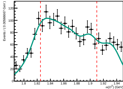
Total ( 0 < n_{\text{Tracks}} < 200 , 3.6 < \eta < 5.0 , 60000 < p < 100000 )
