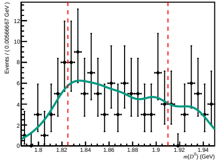
Failed ( 0 < n_{\text{Tracks}} < 200 , 3.6 < \eta < 5.0 , 60000 < p < 100000 )
