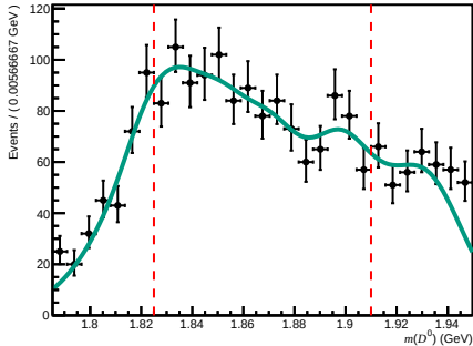
Passed ( 0 < n_{\text{Tracks}} < 200 , 3.6 < \eta < 5.0 , 60000 < p < 100000 )
