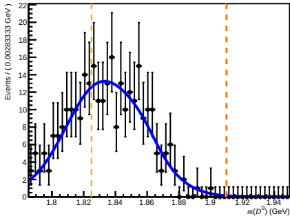
Passed DIF (before RICH1) ( 0 < nTracks < 200 , 3.6 < \eta < 5.0 , 60000 < p < 100000 )
