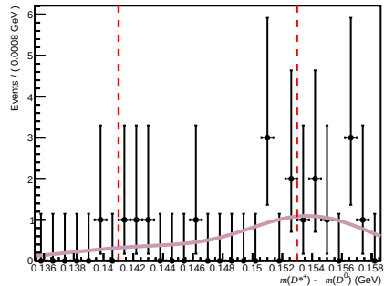
Total ( 200 < n\text{Tracks} < 600 , 1.7 < \eta < 3.6 , 3000 < p < 6000 )
