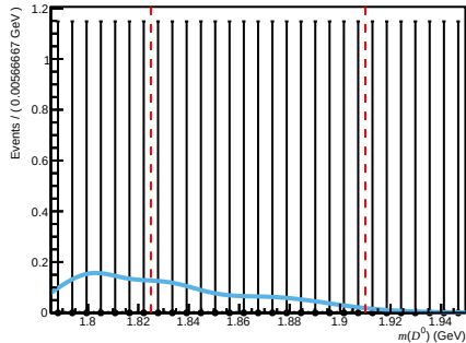
Passed ( 200 < n\text{Tracks} < 600 , 1.7 < \eta < 3.6 , 6000 < p < 10000 )
