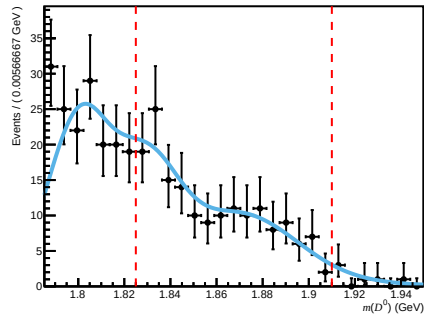
Total ( 200 < n\text{Tracks} < 600 , 1.7 < \eta < 3.6 , 6000 < p < 10000 )
