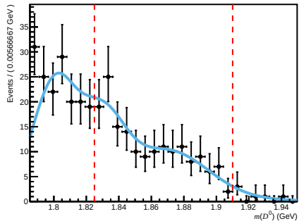
Failed ( 200 < n\text{Tracks} < 600 , 1.7 < \eta < 3.6 , 6000 < p < 10000 )
