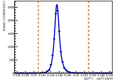
Failed DIF ( 200 < nTracks < 600 , 1.7 < \eta < 3.6 , 6000 < p < 10000 )
