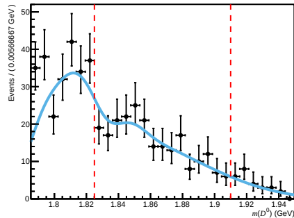
Total ( 200 < nTracks < 600 , 1.7 < \eta < 3.6 , 10000 < p < 15600 )
