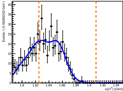
Passed DiF (before RICH1) ( 200 < n_{\text{Tracks}} < 600 , 1.7 < \eta < 3.6 , 27000 < p < 60000 )
