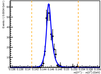
Passed DiF (after RICH1) ( 200 < n\text{Tracks} < 600 , 1.7 < \eta < 3.6 , 60000 < p < 100000 )
