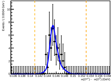
Passed DiF (before RICH1) ( 200 < n\text{Tracks} < 600 , 1.7 < \eta < 3.6 , 60000 < p < 100000 )
