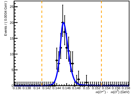
Failed DiF ( 200 < n\text{Tracks} < 600 , 1.7 < \eta < 3.6 , 60000 < p < 100000 )
