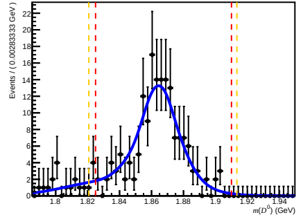
Failed DiF ( 200 < nTracks < 600 , 3.6 < \eta < 5.0 , 3000 < p < 6000 )
