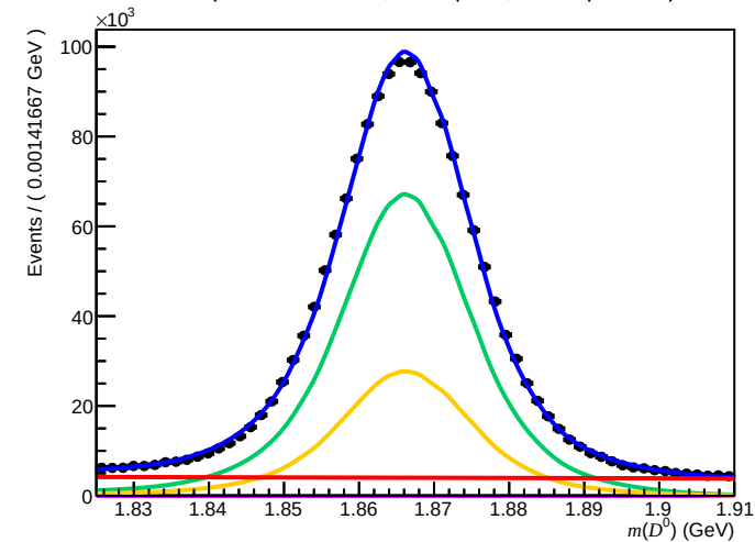
Failed ( 200 < n\text{Tracks} < 600 , 3.6 < \eta < 5.0 , 15600 < p < 27000 )
