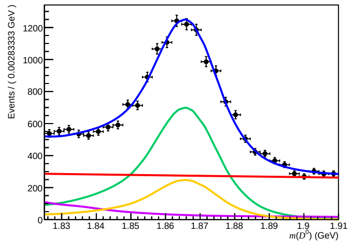
Failed ( 200 < n\text{Tracks} < 600 , 3.6 < \eta < 5.0 , 15600 < p < 27000 )
