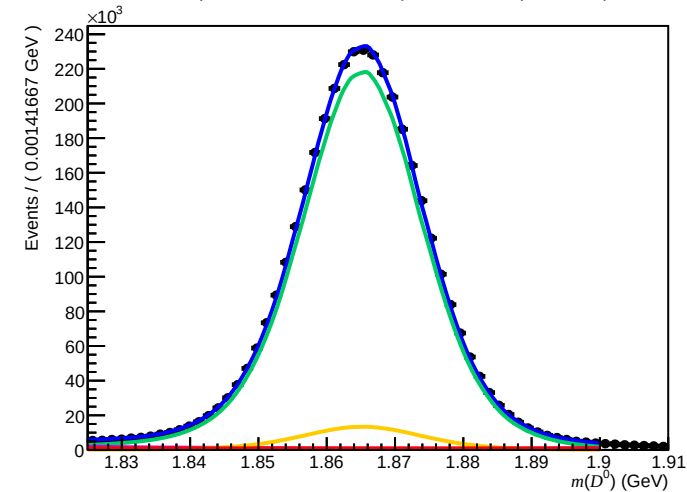
Failed ( 0 < n_{\text{Tracks}} < 200 , 1.7 < \eta < 3.6 , 60000 < p < 100000 )
