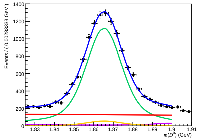
Passed ( 0 < n_{\text{Tracks}} < 200 , 1.7 < \eta < 3.6 , 60000 < p < 100000 )
