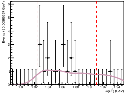
Passed ( 0 < n_{\text{Tracks}} < 200 , 3.6 < \eta < 5.0 , 6000 < p < 10000 )
