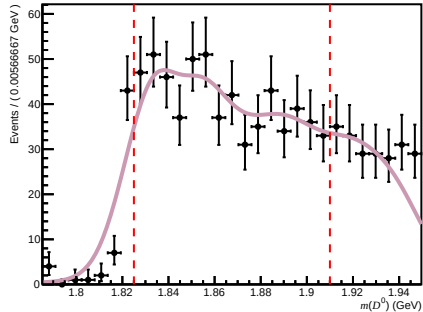
Failed ( 0 < n_{\text{Tracks}} < 200 , 3.6 < \eta < 5.0 , 6000 < p < 10000 )
