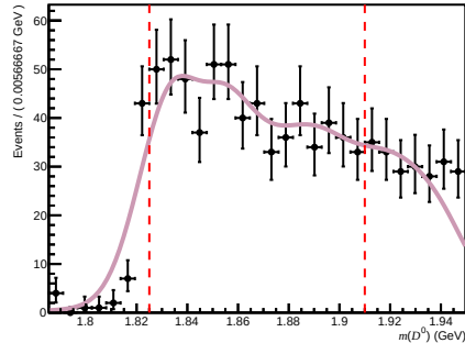
Total ( 0 < n_{\text{Tracks}} < 200 , 3.6 < \eta < 5.0 , 6000 < p < 10000 )
