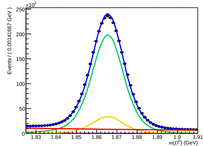
Failed ( 0 < n_{\text{Tracks}} < 200 , 3.6 < \eta < 5.0 , 15600 < p < 27000 )
