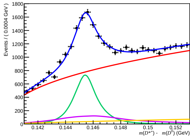
Passed ( 0 < n_{\text{Tracks}} < 200 , 3.6 < \eta < 5.0 , 15600 < p < 27000 )
