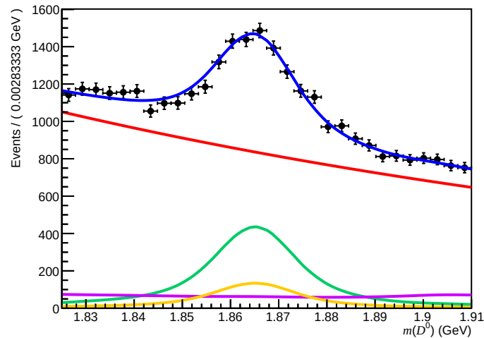
Passed ( 0 < n_{\text{Tracks}} < 200 , 3.6 < \eta < 5.0 , 15600 < p < 27000 )
