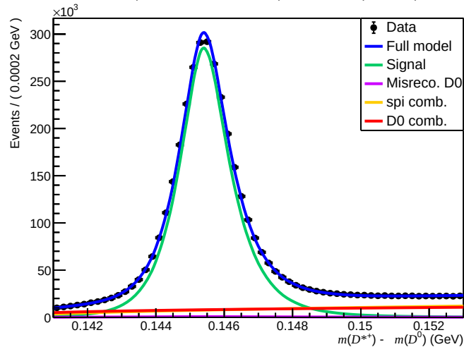
Failed ( 0 < n_{\text{Tracks}} < 200 , 3.6 < \eta < 5.0 , 15600 < p < 27000 )
