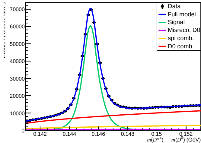
Failed (200 < nTracks < 600, 1.7 < \eta < 3.6, 3000 < p < 6000)
