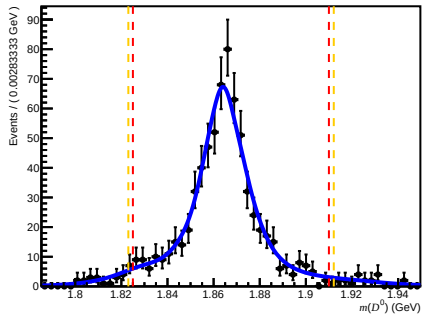
Passed DIF (after RICH1) ( 200 < nTracks < 600 , 1.7 < \eta < 3.6 , 6000 < p < 10000 )
