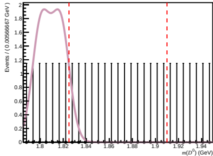
Passed ( 200 < n\text{Tracks} < 600 , 3.6 < \eta < 5.0 , 60000 < p < 100000 )
