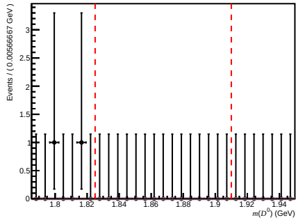
Failed ( 200 < n\text{Tracks} < 600 , 3.6 < \eta < 5.0 , 60000 < p < 100000 )
