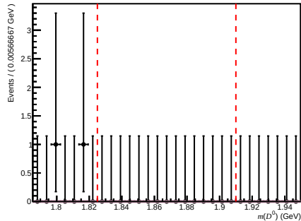
Total ( 200 < n\text{Tracks} < 600 , 3.6 < \eta < 5.0 , 60000 < p < 100000 )
