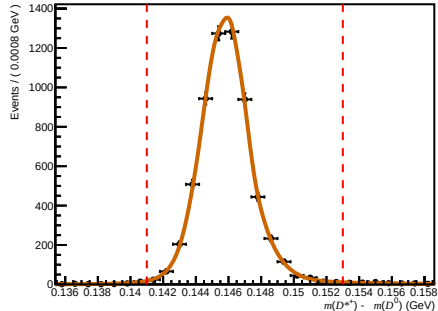
Total ( 0 < n_{\text{Tracks}} < 200 , 1.7 < \eta < 3.6 , 3000 < p < 6000 )
