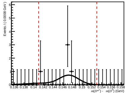
Total ( 0 < n_{\text{Tracks}} < 200 , 1.7 < \eta < 3.6 , 6000 < p < 10000 )
