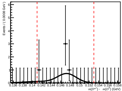
Failed ( 0 < n_{\text{Tracks}} < 200 , 1.7 < \eta < 3.6 , 6000 < p < 10000 )
