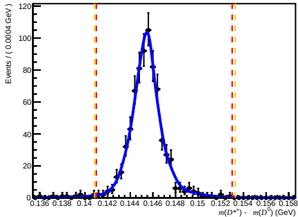
Passed DiF (before RICH1) ( 0 < nTracks < 200 , 3.6 < \eta < 5.0 , 10000 < p < 15600 )
