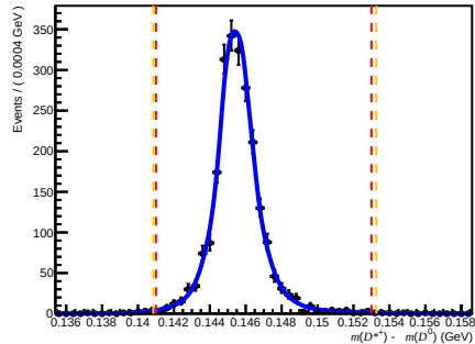
Failed DiF ( 0 < nTracks < 200 , 3.6 < \eta < 5.0 , 10000 < p < 15600 )
