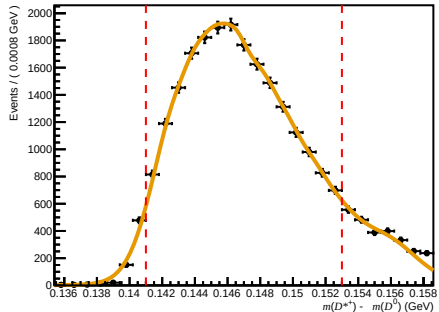
Failed ( 0 < nTracks < 200 , 3.6 < \eta < 5.0 , 27000 < p < 60000 )
