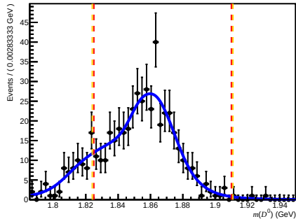
Failed DIF ( 0 < n_{\text{Tracks}} < 200 , 3.6 < \eta < 5.0 , 60000 < p < 100000 )
