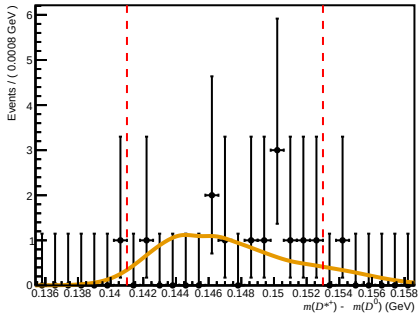
Passed ( 0 < nTracks < 200 , 3.6 < \eta < 5.0 , 60000 < p < 100000 )
