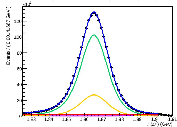
Failed (200 < nTracks < 600, 1.7 < \eta < 3.6, 3000 < p < 6000)
