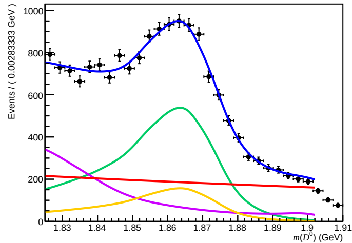
Failed (200 < nTracks < 600, 1.7 < \eta < 3.6, 3000 < p < 6000)
