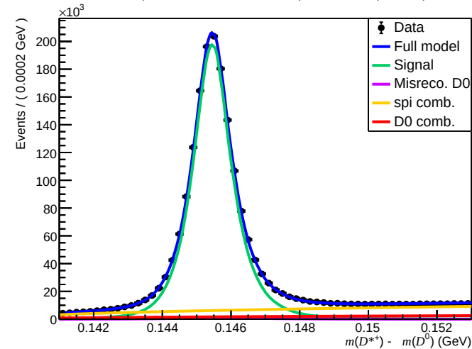
Failed (200 < nTracks < 600, 1.7 < \eta < 3.6, 3000 < p < 6000)
