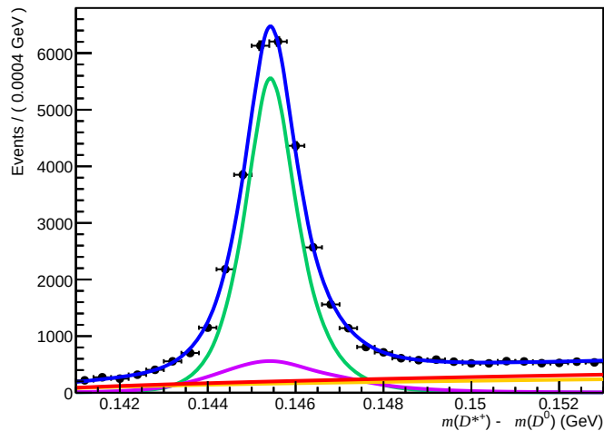
Failed (200 < nTracks < 600, 1.7 < \eta < 3.6, 6000 < p < 10000)
