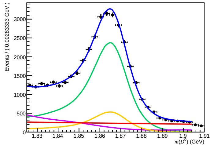
Failed (200 < nTracks < 600, 1.7 < \eta < 3.6, 6000 < p < 10000)
