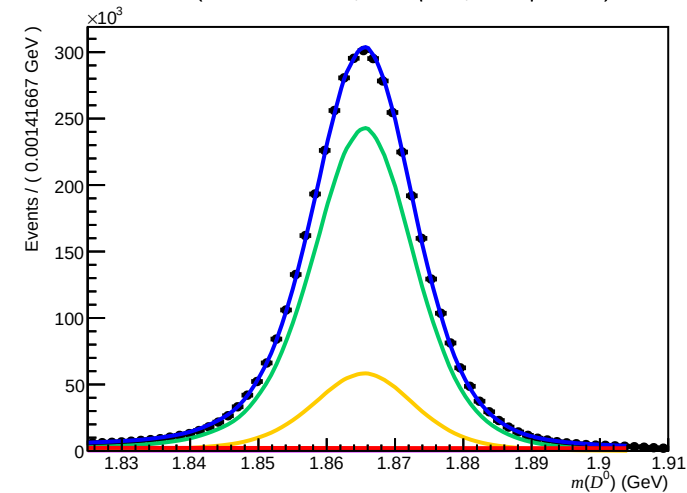
Failed (200 < nTracks < 600, 1.7 < \eta < 3.6, 6000 < p < 10000)
