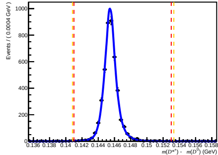
Failed DiF ( 200 < nTracks < 600 , 1.7 < \eta < 3.6 , 10000 < p < 15600 )
