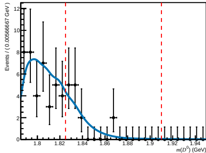
Failed ( 200 < n\text{Tracks} < 600 , 1.7 < \eta < 3.6 , 15600 < p < 27000 )
