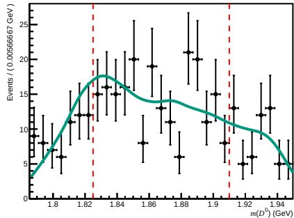
Failed ( 200 < n\text{Tracks} < 600 , 1.7 < \eta < 3.6 , 27000 < p < 60000 )
