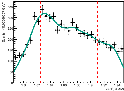
Passed ( 200 < n\text{Tracks} < 600 , 1.7 < \eta < 3.6 , 27000 < p < 60000 )
