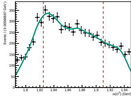
Total ( 200 < n\text{Tracks} < 600 , 1.7 < \eta < 3.6 , 27000 < p < 60000 )
