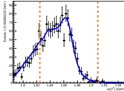
Failed DiF ( 200 < nTracks < 600 , 1.7 < \eta < 3.6 , 27000 < p < 60000 )
