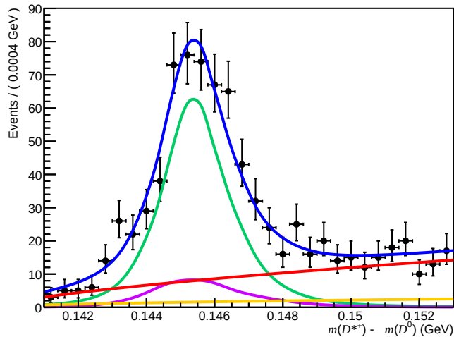
Failed ( 200 < n\text{Tracks} < 600 , 3.6 < \eta < 5.0 , 3000 < p < 6000 )
