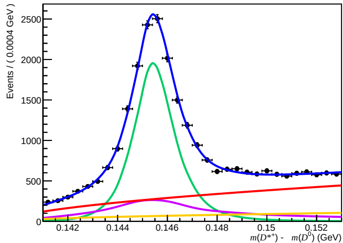
Failed ( 200 < n\text{Tracks} < 600 , 3.6 < \eta < 5.0 , 27000 < p < 60000 )
