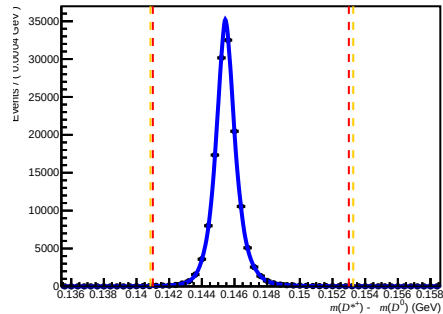
Failed DiF ( 0 < n_{\text{Tracks}} < 200 , 1.7 < \eta < 3.6 , 10000 < p < 15600 )
