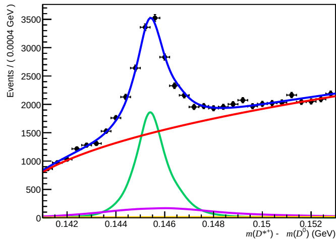
Failed ( 0 < n_{\text{Tracks}} < 200 , 1.7 < \eta < 3.6 , 15600 < p < 27000 )
