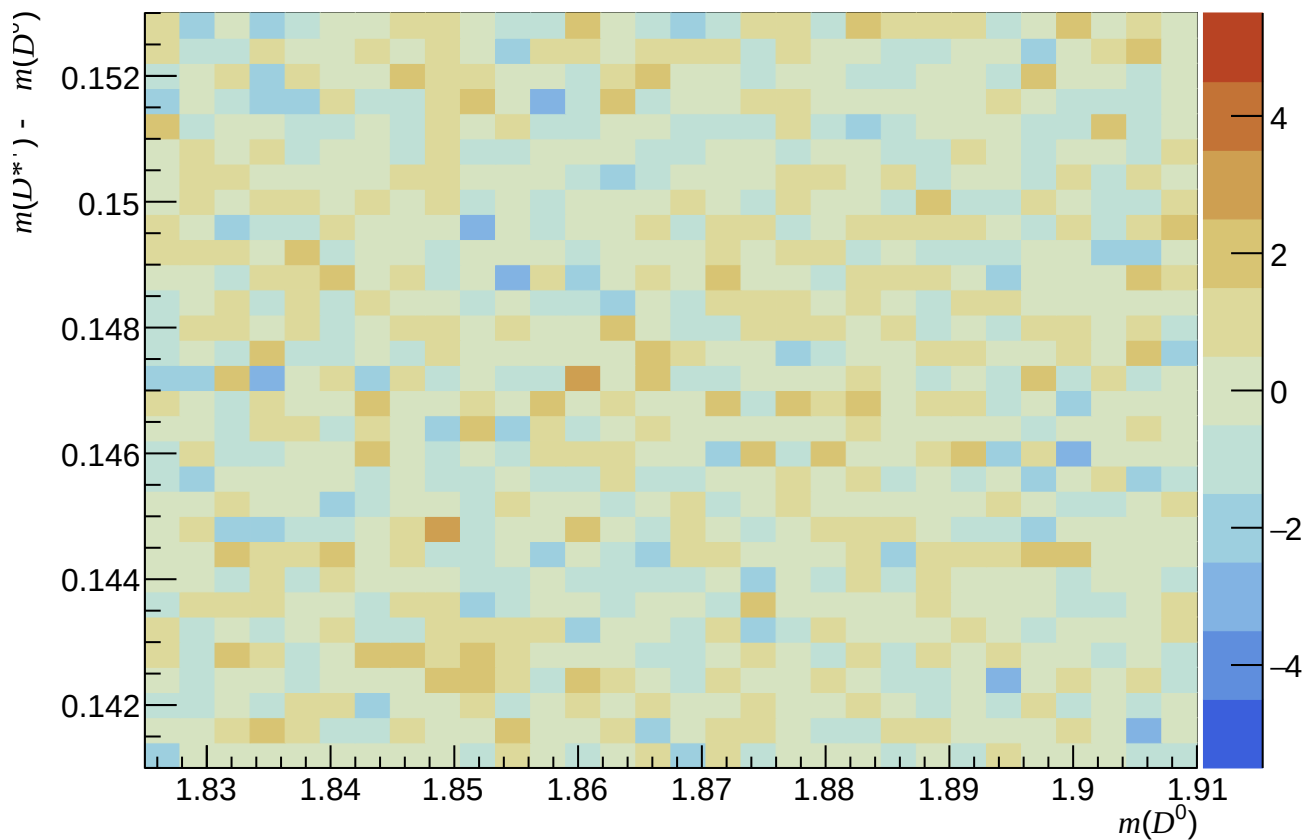
Passed ( 0 < nTracks < 200 , 3.6 < \eta < 5.0 , 15600 < p < 27000 )
