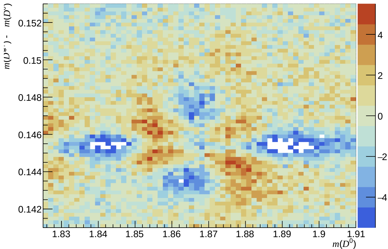
Failed ( 0 < nTracks < 200 , 3.6 < \eta < 5.0 , 15600 < p < 27000 )
