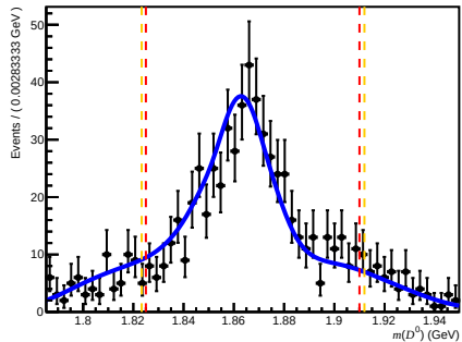
Passed DiF (after RICH1) ( 200 < nTracks < 600 , 1.7 < \eta < 3.6 , 15600 < p < 27000 )
