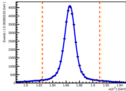
Failed DiF ( 200 < nTracks < 600 , 1.7 < \eta < 3.6 , 15600 < p < 27000 )
