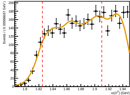
Failed ( 200 < nTracks < 600 , 3.6 < \eta < 5.0 , 3000 < p < 6000 )
