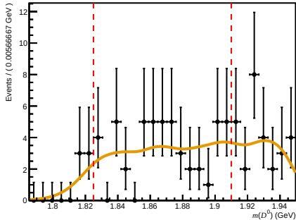
Passed ( 200 < nTracks < 600 , 3.6 < \eta < 5.0 , 3000 < p < 6000 )
