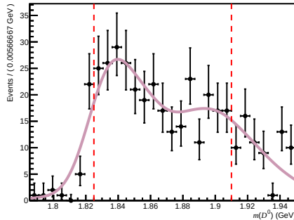
Total ( 200 < nTracks < 600 , 3.6 < \eta < 5.0 , 10000 < p < 15600 )
