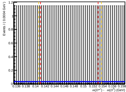
Passed DiF (before RICH1) ( 200 < nTracks < 600 , 3.6 < \eta < 5.0 , 10000 < p < 15600 )
