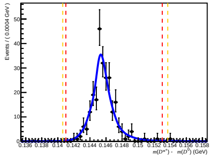
Passed DiF (after RICH1) ( 200 < nTracks < 600 , 3.6 < \eta < 5.0 , 10000 < p < 15600 )
