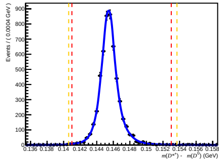
Failed DiF ( 200 < nTracks < 600 , 3.6 < \eta < 5.0 , 10000 < p < 15600 )
