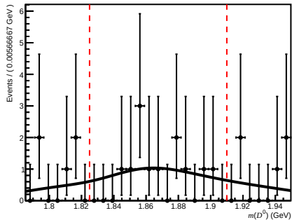
Failed ( 200 < n\text{Tracks} < 600 , 3.6 < \eta < 5.0 , 27000 < p < 60000 )
