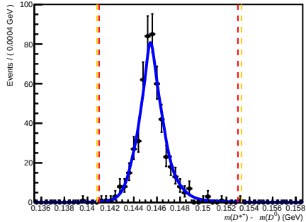
Passed DiF (after RICH1) ( 200 < nTracks < 600 , 3.6 < \eta < 5.0 , 60000 < p < 100000 )
