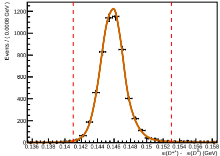
Failed ( 0 < n_{\text{Tracks}} < 200 , 3.6 < \eta < 5.0 , 3000 < p < 6000 )
