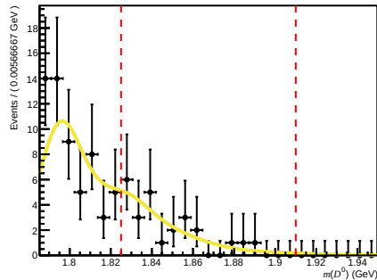
Total ( 0 < n\text{Tracks} < 200 , 3.6 < \eta < 5.0 , 10000 < p < 15600 )
