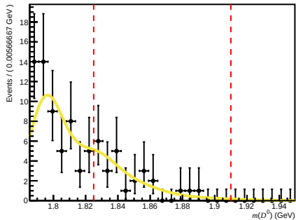
Failed ( 0 < n\text{Tracks} < 200 , 3.6 < \eta < 5.0 , 10000 < p < 15600 )
