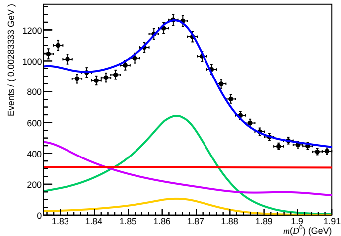
Failed ( 0 < n_{\text{Tracks}} < 200 , 3.6 < \eta < 5.0 , 60000 < p < 100000 )
