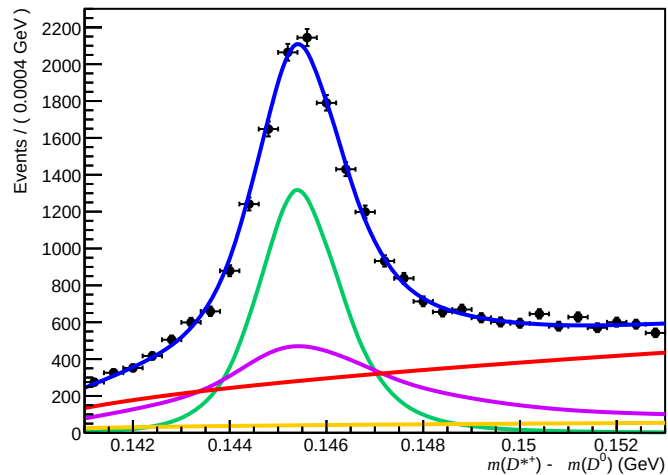
Failed ( 0 < n_{\text{Tracks}} < 200 , 3.6 < \eta < 5.0 , 60000 < p < 100000 )
