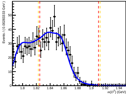
Passed DiF (before RICH1) ( 200 < n\text{Tracks} < 600 , 1.7 < \eta < 3.6 , 3000 < p < 6000 )
