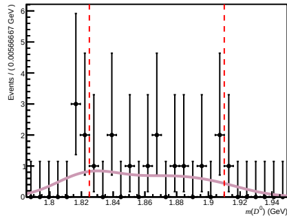
Total ( 200 < nTracks < 600 , 1.7 < \eta < 3.6 , 10000 < p < 15600 )
