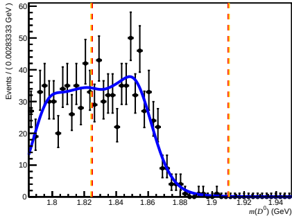
Passed DiF (before RICH1) ( 200 < nTracks < 600 , 1.7 < \eta < 3.6 , 10000 < p < 15600 )
