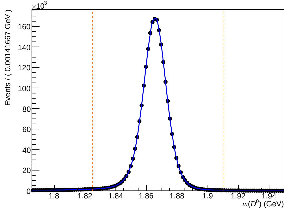
Failed non-DiF ( 200 < nTracks < 600 , 1.7 < \eta < 3.6 , 15600 < p < 27000 )
