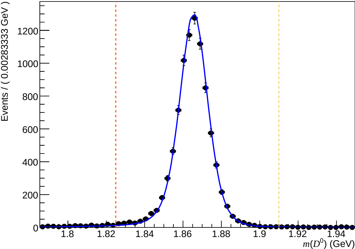
Passed non-DiF ( 200 < nTracks < 600 , 1.7 < \eta < 3.6 , 15600 < p < 27000 )
