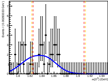
Passed DiF (before RICH1) ( 200 < nTracks < 600 , 1.7 < \eta < 3.6 , 60000 < p < 100000 )
