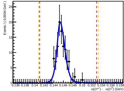
Failed DiF ( 200 < n\text{Tracks} < 600 , 1.7 < \eta < 3.6 , 60000 < p < 100000 )
